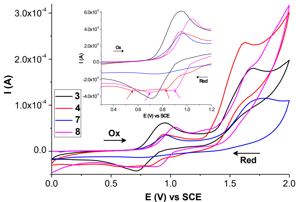
Figure 12. Diagrams of representative mono- and di-substituted phenothiazine dyes, obtained by current sweep in the positive direction
