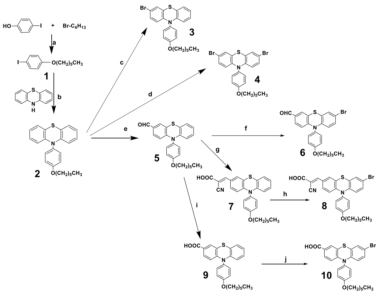
Scheme 1. Phenothiazine derivatives synthesis: (a) DMF, K_2CO_3 , 110-120 °C, 8h; (b) o -dichlorobenzene, copper powder, 18-crown-6, K_2CO_3 , 168 °C, 24h; (c), (d), (f), (h) NBS, CHCl_3 , CH_3COOH , 0 °C, 2h; (e) DMF, POCl_3 , C_2H_4Cl_2 , 90 °C, 24h; (g) cyanoacetic acid, piperidine, acetonitrile, 80 °C, 24h; (i) THF, t -BuOK, 0 °C, RT, 24h; (j) NBS, DMF, 0 °C, 2h.
