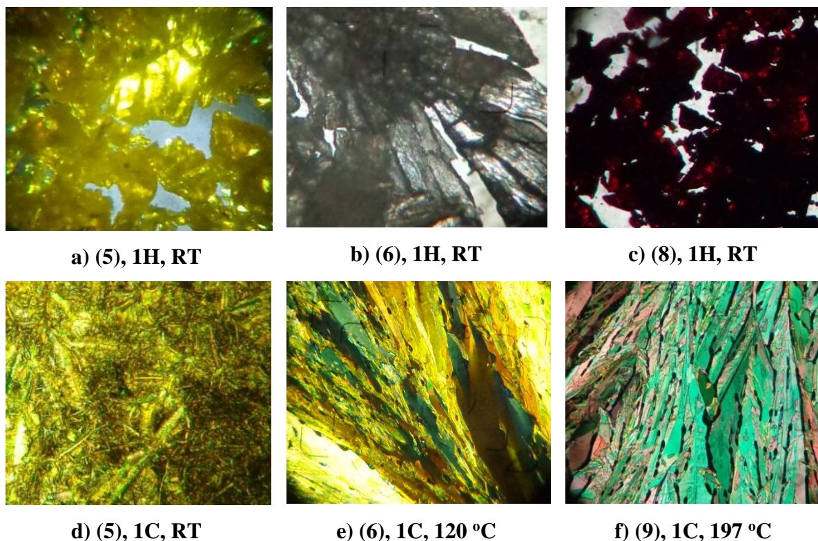
Figure 7. POM images (magnification 200x, C: cooling; H: heating)
