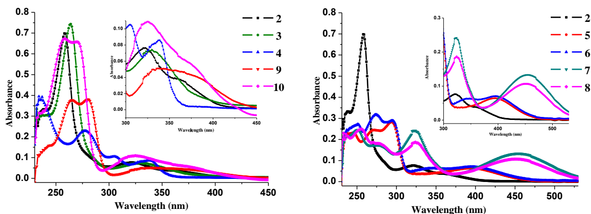
Figure 8. UV-vis absorption spectra, in THF solutions ( 10^{-5}\text{M} ) (the inset represents the magnification of the absorption domain over 300 nm)
